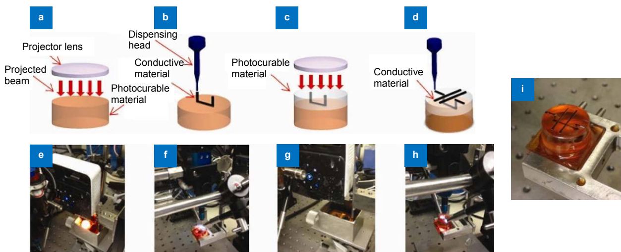
Fig. 7 | The hybrid 3D printing process and fabricated 3D structural electronics. (a) Bottom insulating structure. (b) "U" shape wire. (c) Top insulating layer. (d) Wires on top surface. (e) PμSL of the bottom insulating structure. (f) DWC of the "U" shape wire. (g) PμSL of the top insulating structure. (h) DWC of wires on the top surface. (i) Fabricated 3D structural electronics with embedded wires. Figure reproduced from ref. 10 , Springer International Publishing AG.
