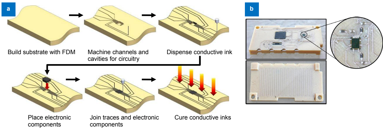
Fig. 2 | (a) Process flow of the multi 3D system. (b) Fabricated parts. Figure adapted from ref. 9 , Springer International Publishing AG.
