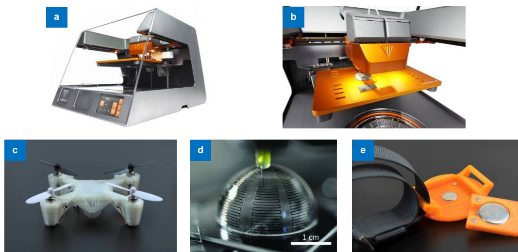
Fig. 13 | Voxel8 and some printed products. (a, b) Photograph of Voxel8 3D printer. (c) Printed unmanned aerial vehicle. (d) Printed antenna (dome). (e) Printed wearable device. Figure reproduced from ref. 32 , Voxel8.
