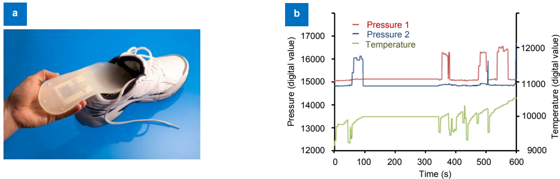
Fig. 4 | (a) Printed wireless pressure and temperature sensor within a shoe's insole. (b) Pressure and temperature data obtained through wireless communication from the printed insole. Figure reproduced from ref. 22 , Society for Imaging Science and Technology.
