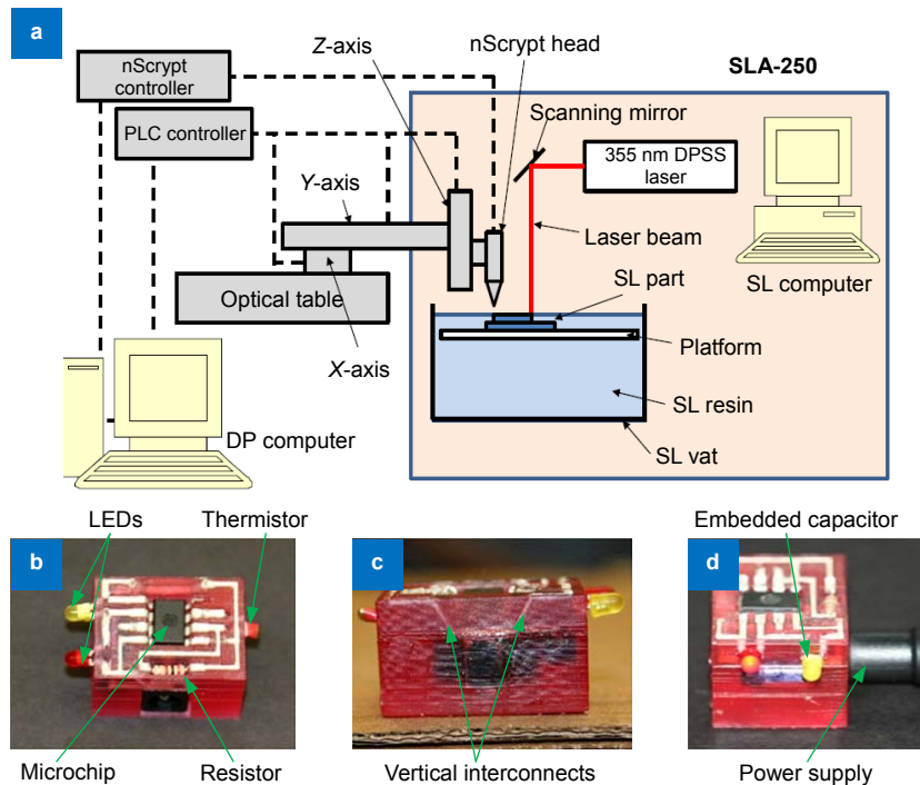
Fig. 6 | (a) Schematic of the hybrid SL/DP system. (b–d) Fabricated 3D 555 timer circuits packaged within SL substrates. Figure reproduced from: (b–d) ref. 24 , Emerald Publishing Limited.
