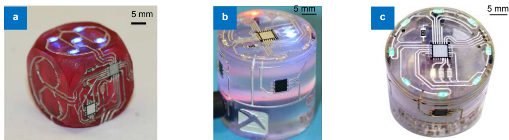
Fig. 8 | Examples of printed 3D structural electronics. (a) A gaming die which includes a microcontroller and accelerometer. (b, c) A magnetometer system with microprocessor and orthogonal Hall Effect sensors. Figure reproduced from ref. 18 , Taylor & Francis.
