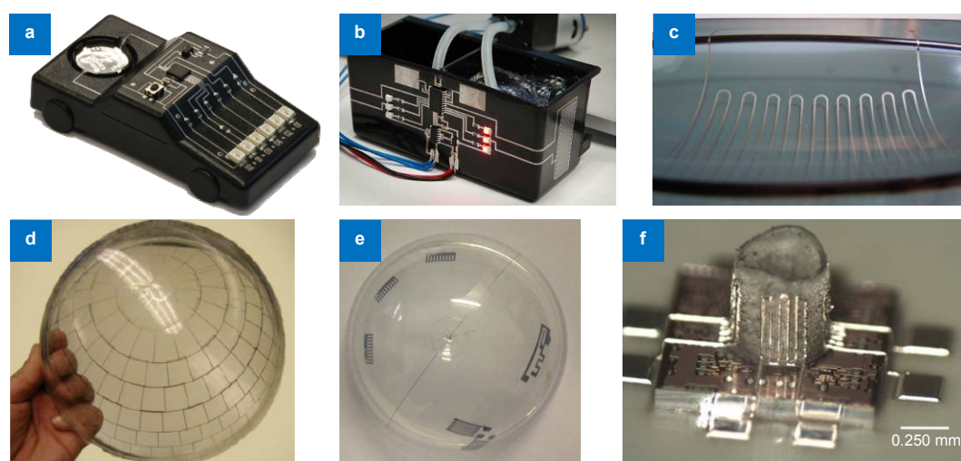
Fig. 11 | 3D printed electronics using Aerosol Jet printing from Optomec. (a) 3D MID demonstrator. (b) 3D MID with integrated sensor. (c) Printed conformal electronics (curve). (d) Printed conformal electronics (dome). (e) Printed conformal electronics (dome). (f) Sub-mm length scale, custom made 3D metal-dielectric. Figure reproduced from (a–c) ref. 28 , Neotech; (d–f) ref. 29 , Optomec.
