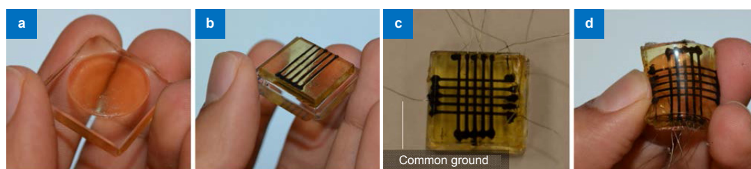
Fig. 10 | Fabricated stretchable tactile sensor using integrated PSL and DP processes. (a) An example (partial sphere) of 3D structure built in the PSL system. (b) Printed sensing elements using the DP process on the insulating layers built in the PSL system. (c) Final sensor with two sensing layers. (d) Deformed sensor. Figure reproduced from ref. 27 , Wiley-VCH Verlag GmbH & Co. KGaA, Weinheim.
